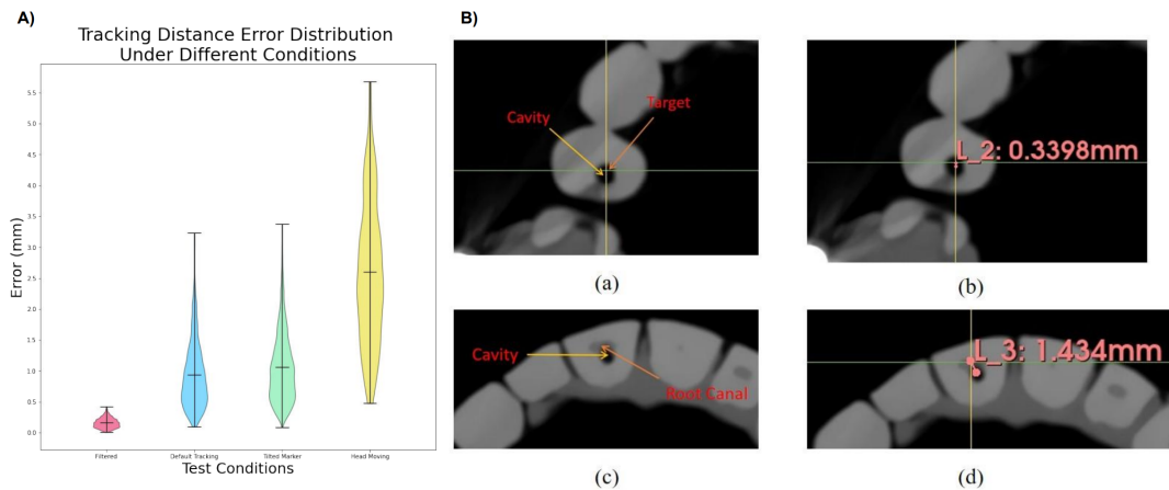
FIGURE 5 A) The error distribution of HoloLens 2-based marker tracking using STTAR. Notice that there were significant errors induced by head motions while tilting the marker to \pm 60 deg had a limited impact on the error. The central dash lines are the mean errors, and the top/bottom dashes are the max/min errors. B) (a) Transverse cross-section that shows cavity and target, where the black hole is the cavity and the cross intersection is the target. (b) The distance deviation of the cavity from the target using the mixed reality method. (c) The transverse cross-section shows the cavity and target, where the black hole is the cavity and the cross intersection is the root canal that represents the target. (d) The distance deviation of the cavity from the target using the freehand method.
