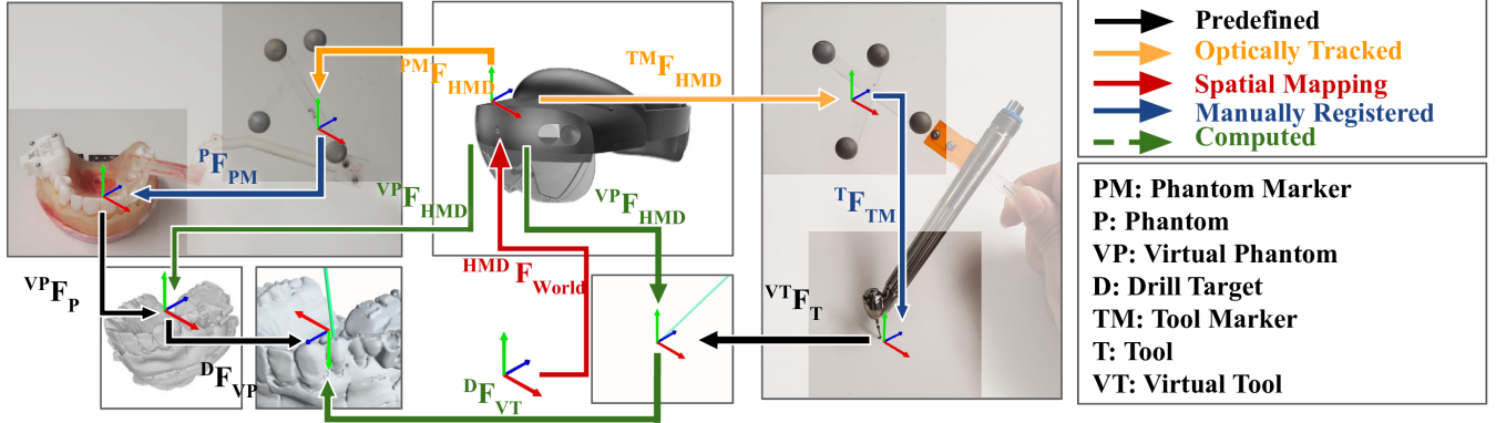
FIGURE 2 The Spatial Relations among the Objects. It should be noted although only one virtual object pair ( VP and VT ) is included in the figure, it is possible to include multiple sets of virtual object pairs ( \{VP_i, VT_i\} ) for different display purposes (e.g., virtual mirrors showing coronal, sagittal, and transverse views, respectively). They would differ in the defined {}^P F_{VP_i} and {}^{VF_i} F_{VT_i} , which orients the virtual object to a desired view pose.
