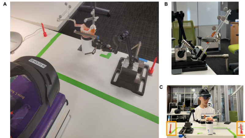
FIGURE 4 A) General setup for evaluating the tracking accuracy of the HoloLens 2 system. B) The setup of the tracker when tilted 45^\circ vertically. Other rotations are done in the same manner. C: The setup for testing the effects of head motion. The test user was instructed to shake his head and to move his view between the two markers (marked in orange boxes).
